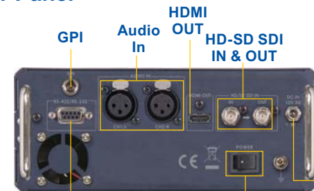
RS-422/RS-232 Power DC In 12V 4.2A
